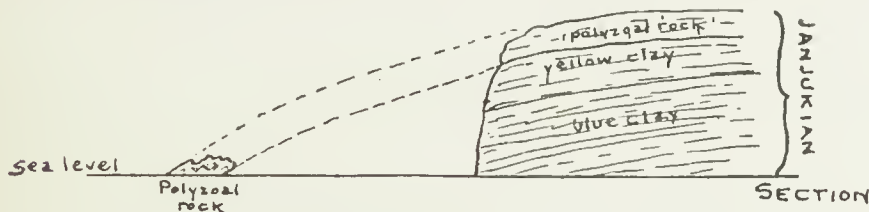
Fig. 8. NEAR SUMMIT OF ANTICLINE AT CURLEWIS (Ad 12), LOOK- ING E: SHOWING POLYZOAL ROCK AS A REEF AT LOW TIDE.
