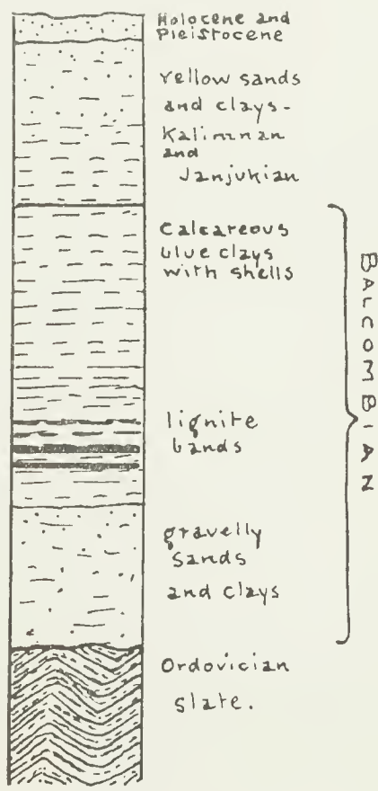
DIAGRAM SECTION OF BORES NEAR ALTONA BAY, PORT PHILLIP.
