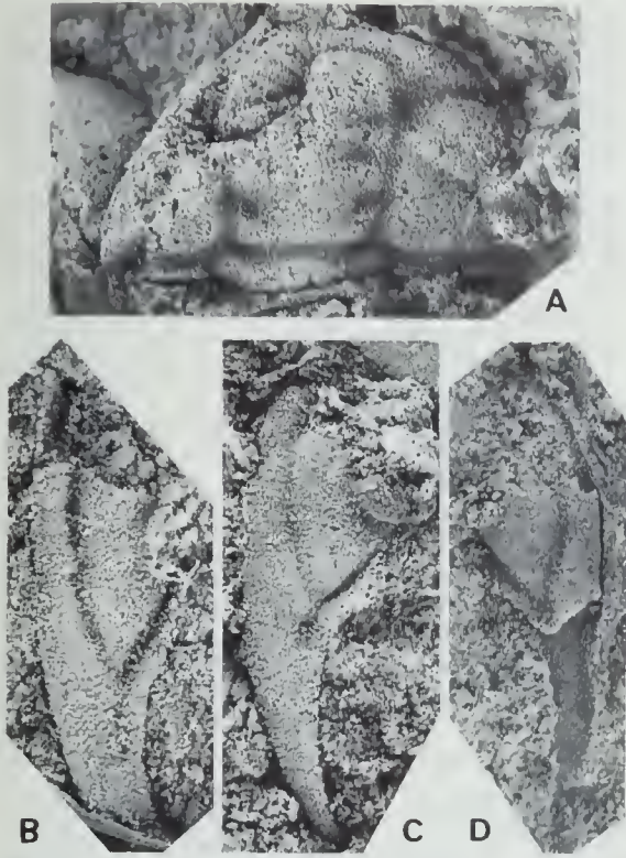
Figure 3. Tasmanocephalus stephensi (Etheridge, 1883). A, internal mould of cranium Z1379, \times 4 . (Figured by Etheridge, 1883, pl. 1, fig. 2 and by Kobayashi, 1936, pl. 21, fig. 2). The librigena illustrated by Etheridge is evident but at a steeper angle to the cranium than originally depicted—see explanation in text. B, latex cast of librigena showing forward extension of the doublure, NMVP71239, \times 4 . C, latex cast of librigena NMVP71240, \times 3 . D, internal mould of librigena showing forward extension of the doublure NMVP71241, \times 3 .
